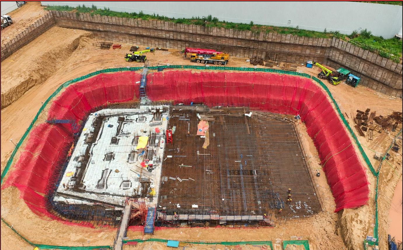
Tower D Raft Reinf. Work in Progress
