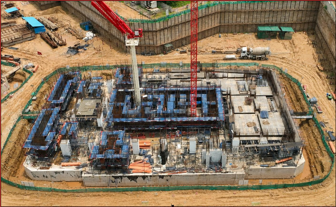
Tower A B3 Level Work in Progress
