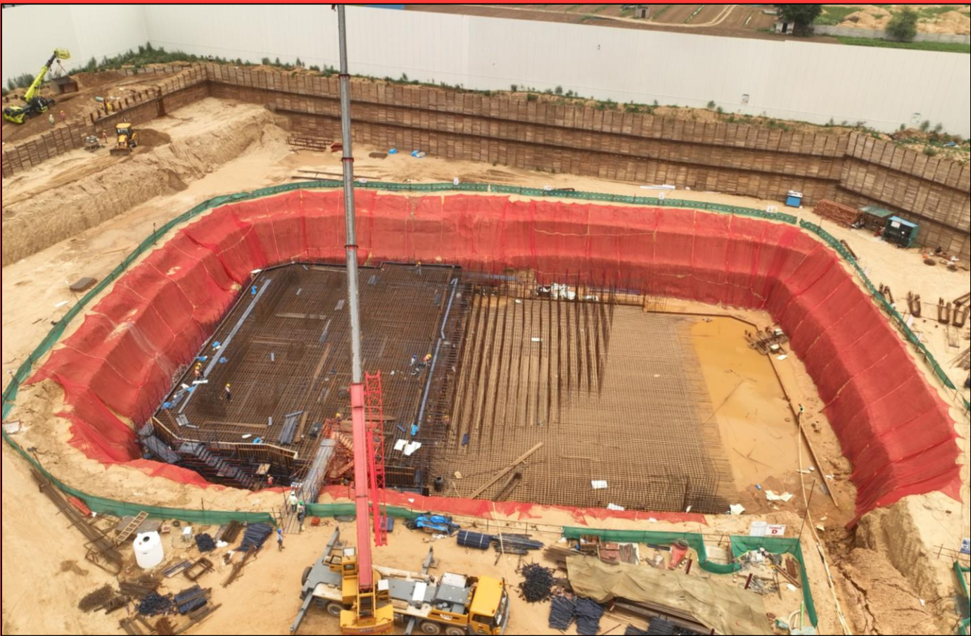
Tower D Raft Reinf. Work in Progress
