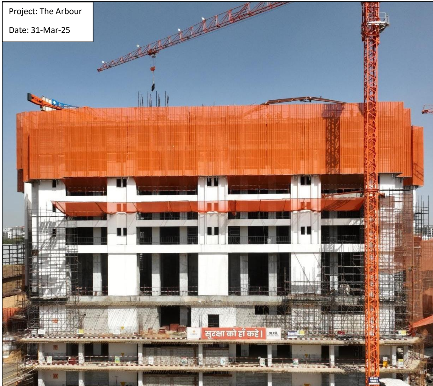
Tower D – 7F Slab WIP
